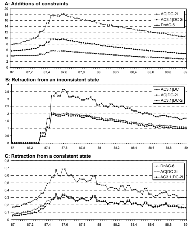
Figure 5. Runtime (in seconds) as a function of tightness in RCSP \langle 100, 50, 0.5, p_2 \rangle .
