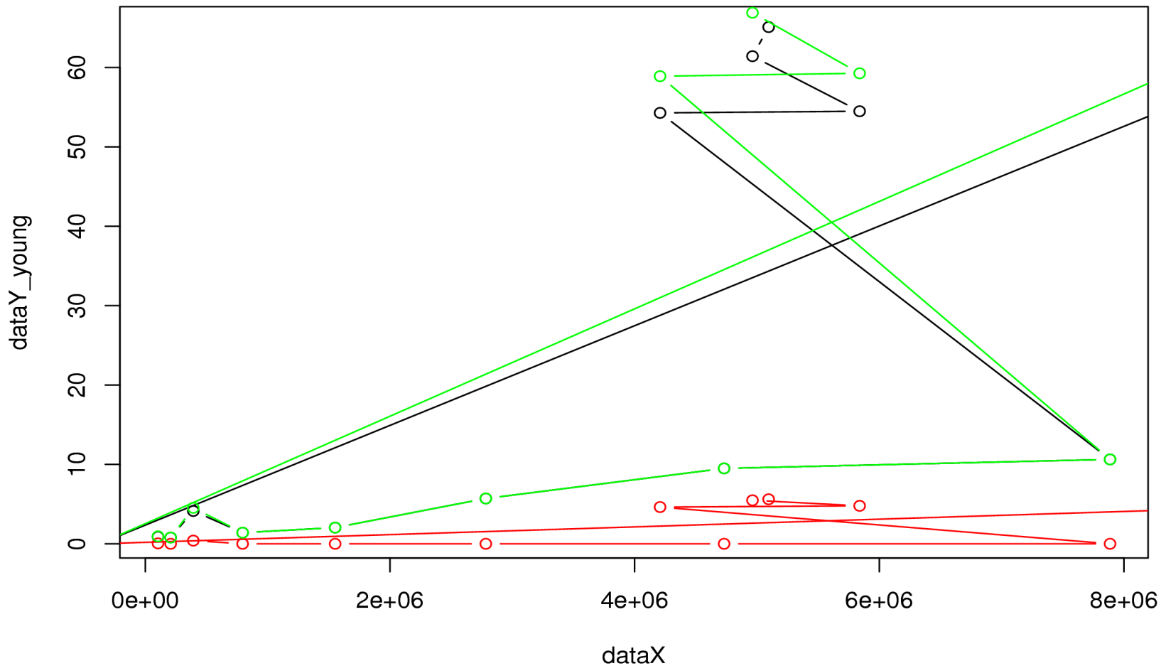
depth.weak.deep.128
